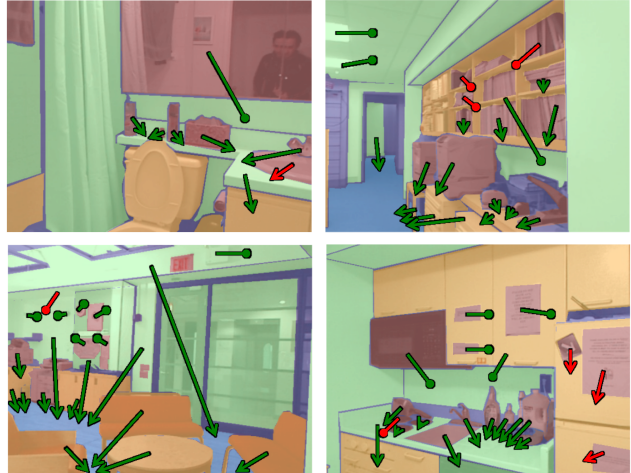
Figure 6. Sample support relation predictions from our model on the NYU Depth v2 dataset [28]. \rightarrow : support from below, \dashrightarrow : support from behind. Red arrows are incorrect predictions. We also color code structure classes: ground is in blue, structure is in green, furniture is in yellow, prop is in red. Purple indicates missing structure class. Note that the segmentation masks are only shown for visualization purpose.
