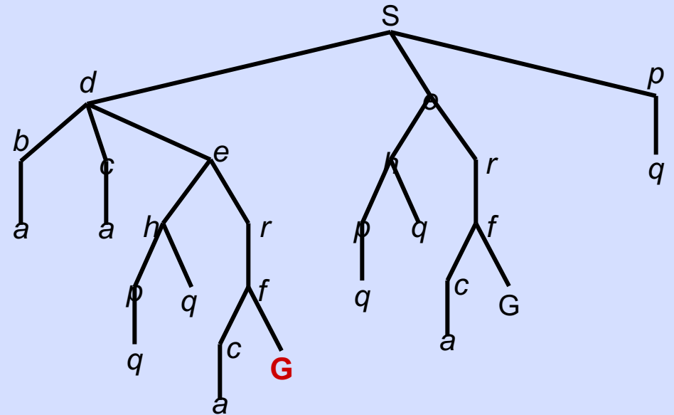
Search Tree
